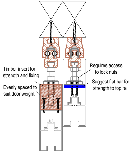
OVERHEAD SCREW FIXING TWO TRACKS (ALUMINIUM DOORS)
