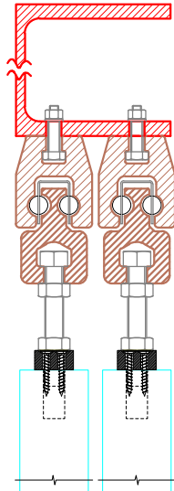
OVERHEAD BOLT FIXING TWO TRACKS
