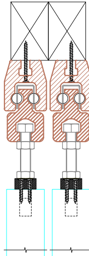
OVERHEAD SCREW FIXING TWO TRACKS (TIMBER DOORS)
