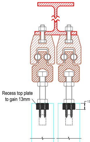
OVERHEAD BOLT FIXING TWO TRACKS
