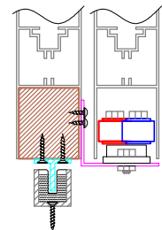
NRC GUIDE COMPLETE WITH STAINLESS STEEL CONNECTING GUIDE
