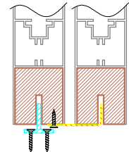
NRC GUIDE COMPLETE WITH STAINLESS STEEL CONNECTING GUIDE
