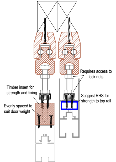
OVERHEAD SCREW FIXING TWO TRACKS (ALUMINIUM DOORS)
