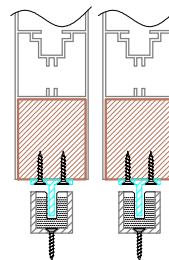
NYLON RECESSED CHANNEL GUIDE (NRC) WITH 2 BRASS TEE GUIDE PER DOOR
