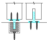
BRASS TEE GUIDE WITH NYLON RECESSED CHANNEL GUIDE
