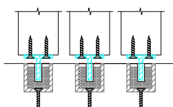
NYLON RECESSED CHANNEL GUIDE (NRC)
