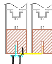
NRC GUIDE COMPLETE WITH STAINLESS STEEL CONNECTING GUIDE
