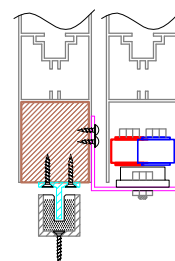
NRC GUIDE COMPLETE WITH STAINLESS STEEL CONNECTING GUIDE
