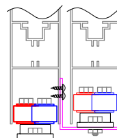
TWIN ROLLER GUIDES COMPLETE WITH STAINLESS STEEL CONNECTING GUIDE
