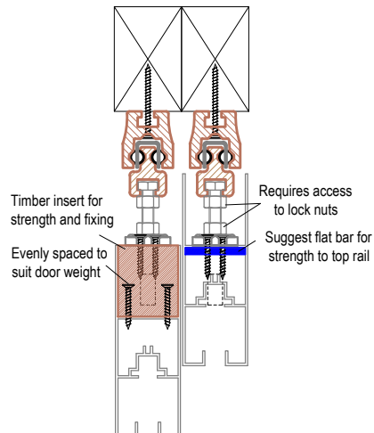
OVERHEAD SCREW FIXING TWO TRACKS (ALUMINIUM DOORS)
