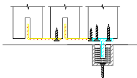
NYLON RECESSED CHANNEL GUIDE WITH STAINLESS STEEL DOOR CONNECTING GUIDES
