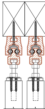
OVERHEAD SCREW FIXING TWO TRACKS (TIMBER DOORS)
