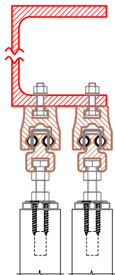
OVERHEAD BOLT FIXING TWO TRACKS
