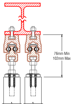
OVERHEAD BOLT FIXING TWO TRACKS
