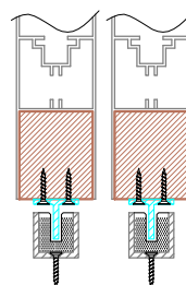
NYLON RECESSED CHANNEL GUIDE (NRC) WITH 2 BRASS TEE GUIDE PER DOOR
