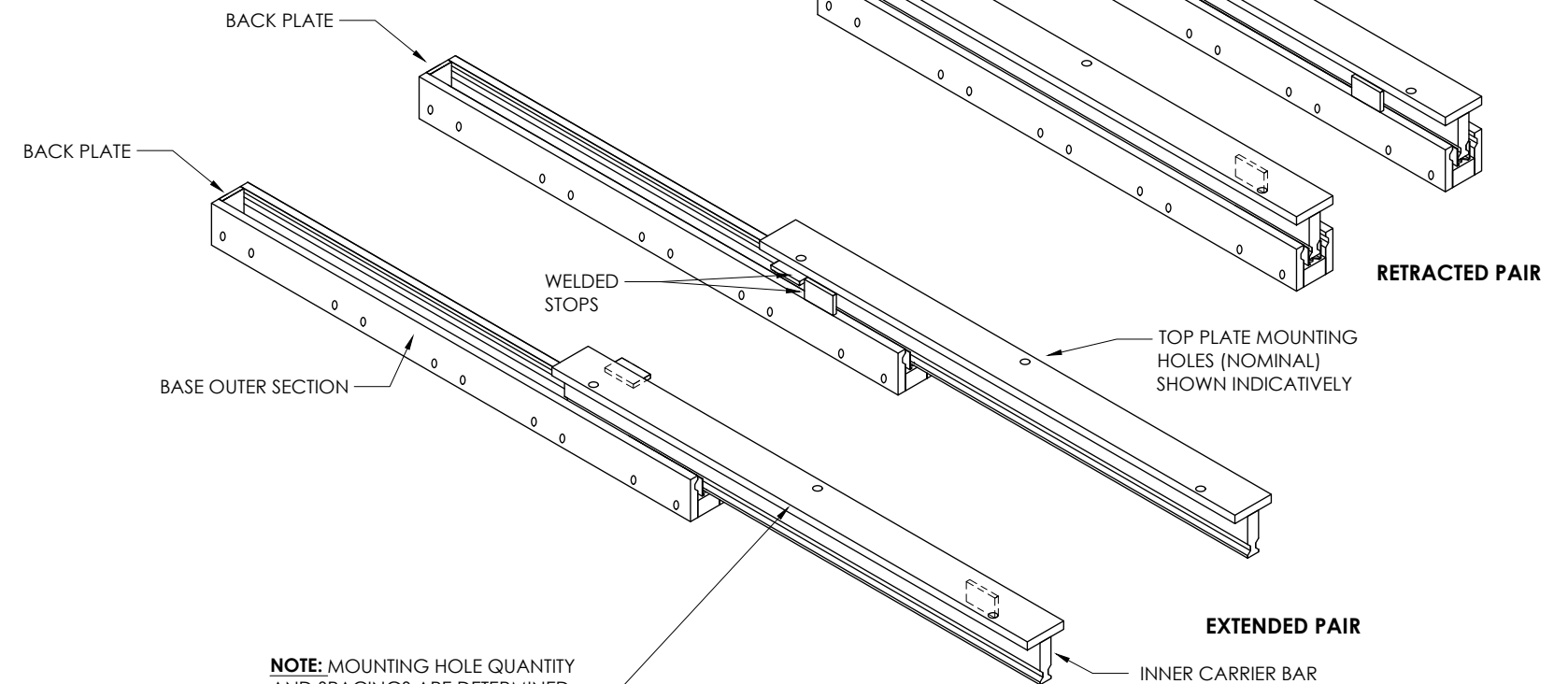
S1000W ISOMETRIC VIEW FOR ILLUSTRATION PURPOSES ONLY DO NOT SCALE
