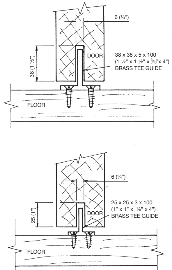
DOOR BASE GUIDES SCALE: HALF FULL SIZE
