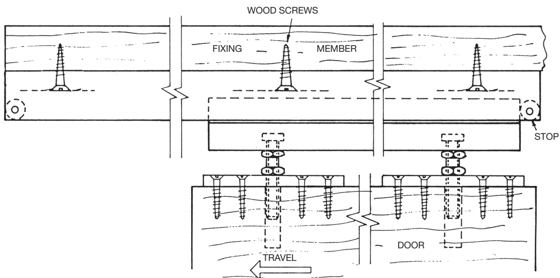
ELEVATION CAVITY FIXING SCALE: QUARTER FULL SIZE
