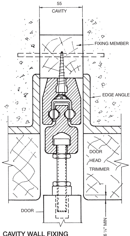
CAVITY WALL FIXING SCALE: HALF FULL SIZE
